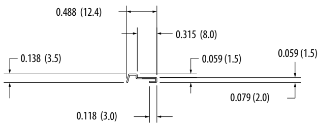
PR2 Channel Guard
