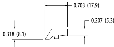
TFW-1/2N (1/2" Wiper w/ Ridge)
