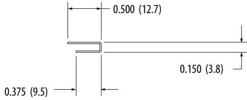
TFC-1/8 (Channel for Wiper TFW-1/8)
