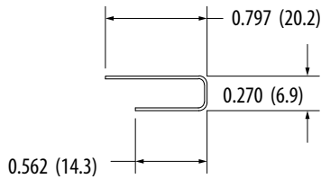
TFC-3/4 (Channel for Wiper TFW-3/4)
