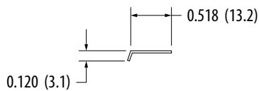
TFG-1/8 (Guard for 1/8" Wiper)
