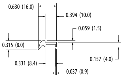
TSA-M16 (TSAM16 Wiper)
