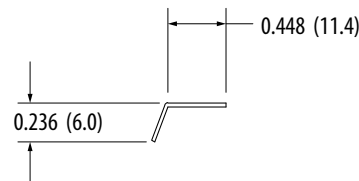
TFG-1/2 & TFG-3/4 (Guard for Wiper TFW-1/2 & TFW-3/4)
