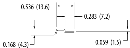
TFG-MA8/N6 (Guard for N6 Wiper/K17593)
