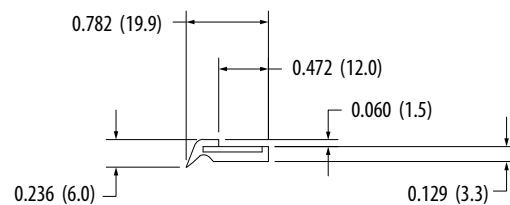
TFW-MA12/N7 (N7 Wiper)
