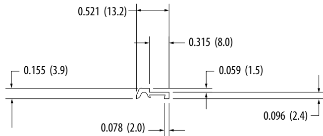
TFCG-741 (Channel & Guard for TFW-740 Wiper)
