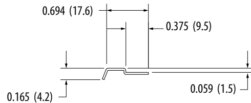
TFG-MA12/N7 (Guard for N7 Wiper/K17592)
