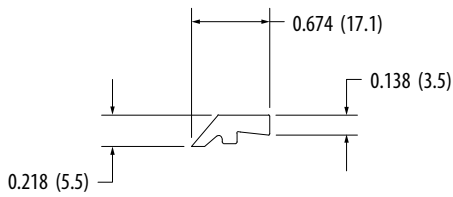
TFW-5/16N (5/16" Wiper w/ Ridge)
