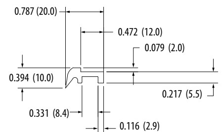
TSA-M19 (TSAM19 Wiper)
