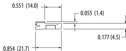
AA00754 Nitta Wiper w/Guard
